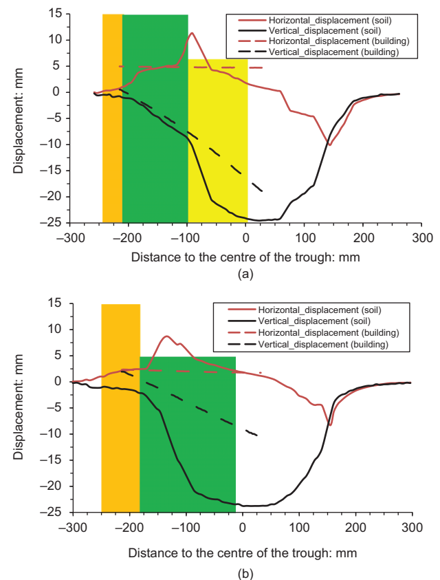
Figure 10. Behaviour of the ground for two different positions of the building: (a) position 1; (b) position 2). Colours show the different cases of soil–structure contact: structure lying on the ground (green), contact lost between structure and ground (orange: rise of the building due to rigid body rotation, yellow: loss of support)
