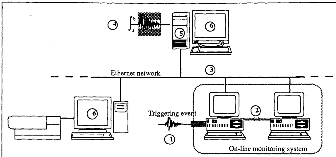
Figure 2: Seismic data acquisition and processing system. 1) event detection; 2) data acquisition on the master PC, switching of the PC to slave mode and pre-processing of the signal; 3) data transmission on multitask machine; 4) complete signal processing; 5) data storage and database type file system update; 6) interactive processing of the events in order to validate the calculated parameters.
