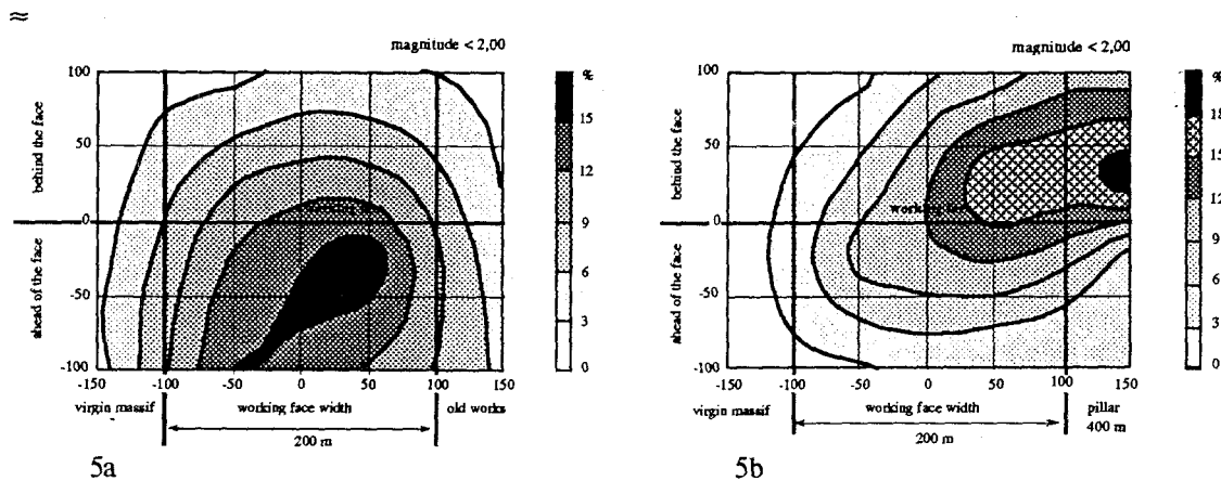
Figure 5: Preferential location of small seismic events (magnitude < 2.0) induced in the course of operation of working face 07 at the North Estaque district, according to two separate operation configurations: a. geometry 1; b. geometry 2.
