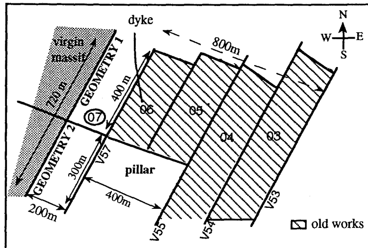
Figure 3: Schematic view of the operation configurations (geometry 1 and geometry 2) for working face 07 in the North Estaque district.
