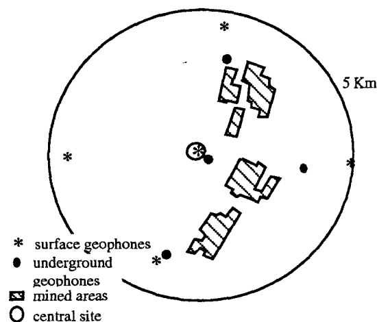
Figure 1: Geometry of the local Provence U.E. seismic network
