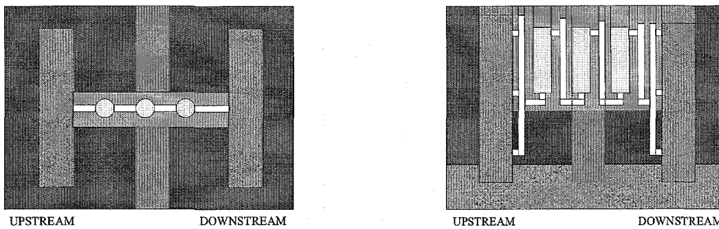
Figures 3a and 3b - Top view and cross-section of the drain panel ®
