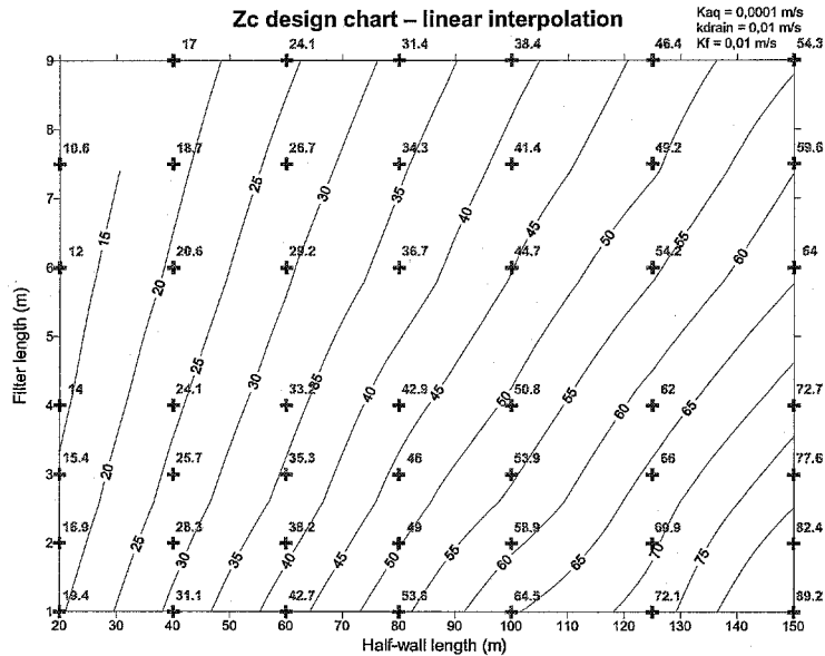
Figure 8 - Example of design chart relating the capture zone, the filter length, and the watertight walls length
