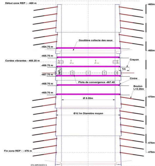
Figure 3. Cross-section of the access shaft (6 m diameter) between -460 m and -475 m
