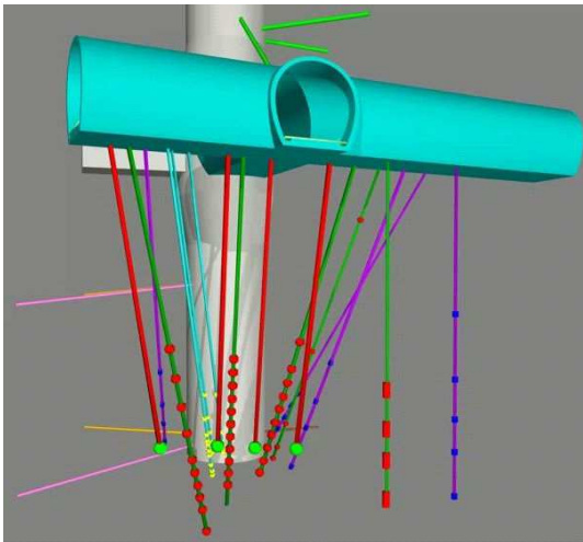
Figure 2. Layout of the REP experiment
