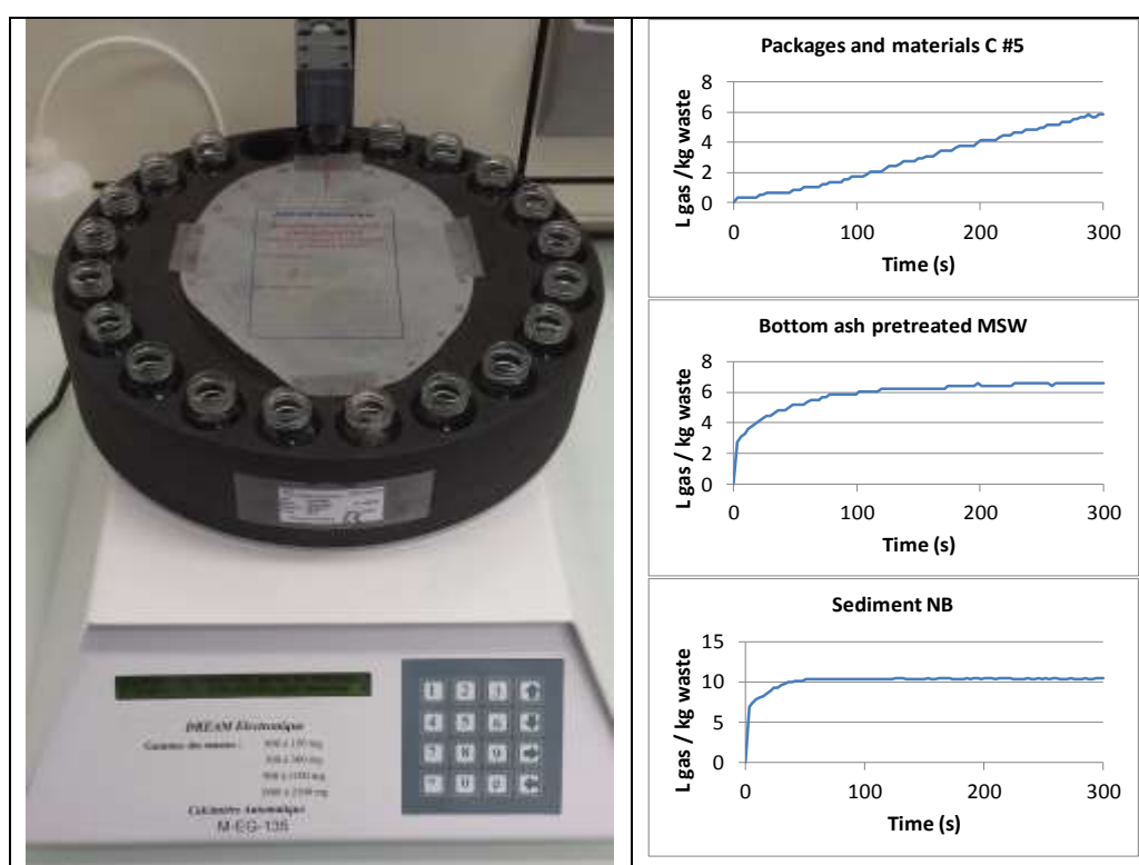
Figure 1: Automatic calcimeter, and example of emission of gas in contact with an acid
