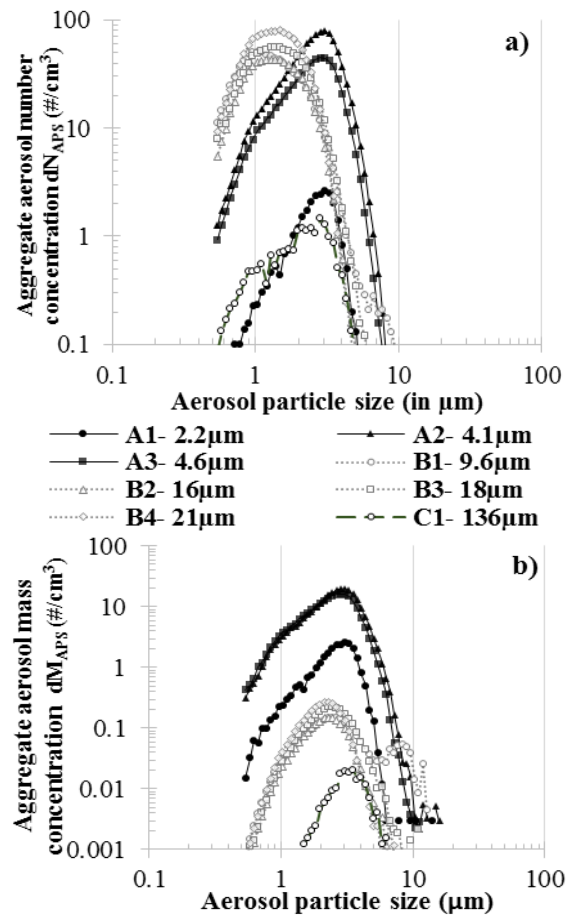
Fig. 3. APS measurements for aggregate aerosol concentration by particle size by a) number concentration (dN); b) mass concentration (dM).
