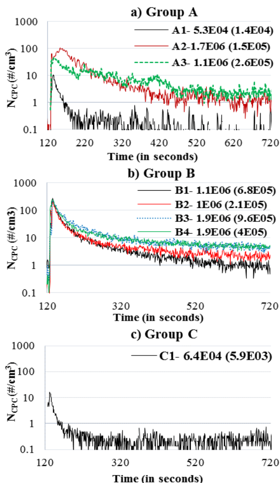
Fig. 2. Temporal evolution of respirable aerosol number concentration from the CPC for a) Group A; b) Group B; c) Group C. The total number of aerosol particles released S_{\text{Total}}^{\text{Number}} and their SD were calculated using (1) and (2) (see top-right corner).
