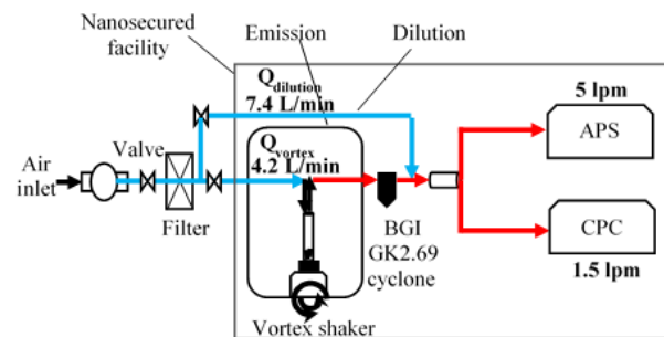
Fig. 1. Schematic of the vortex shaker experimental setup.
