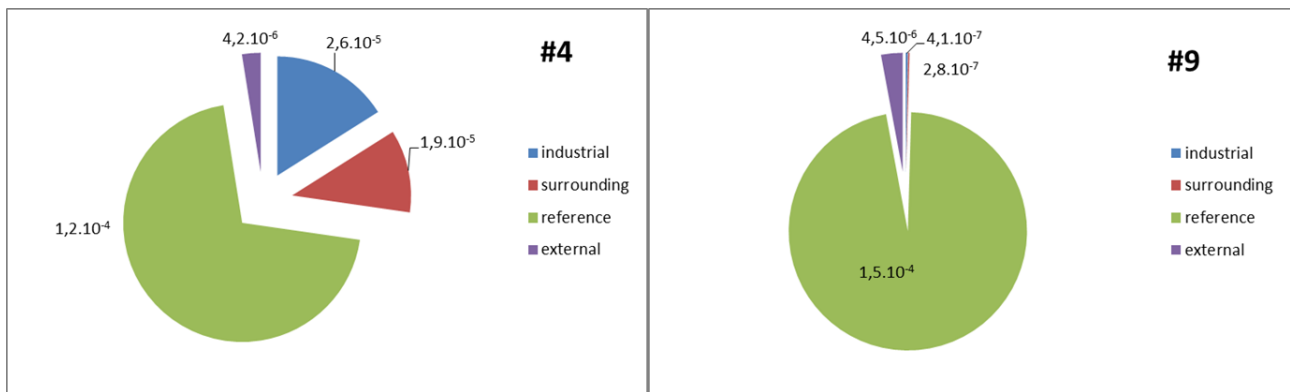
Figure 1: Comparison of the relative contribution of dust ingestion in different areas for 2 different individuals living in the reference area.
