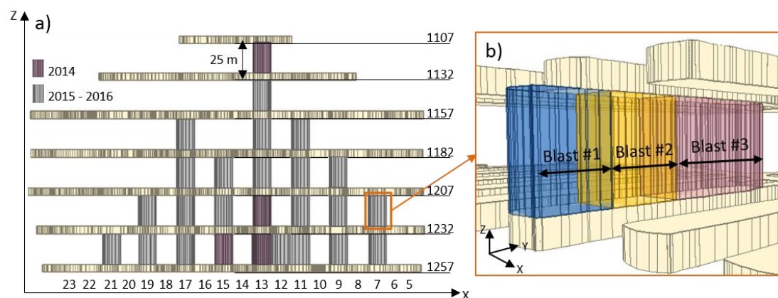
Figure 2. Mining method and sequencing. (a) Vertical profile showing all sub-stopess extracted between 2014 and 2016. Numbers at the bottom indicate stopes' names, while numbers on the right refer to mine's levels. (b) 3D view between two consecutive levels, showing the blast design along the length of a drift.
