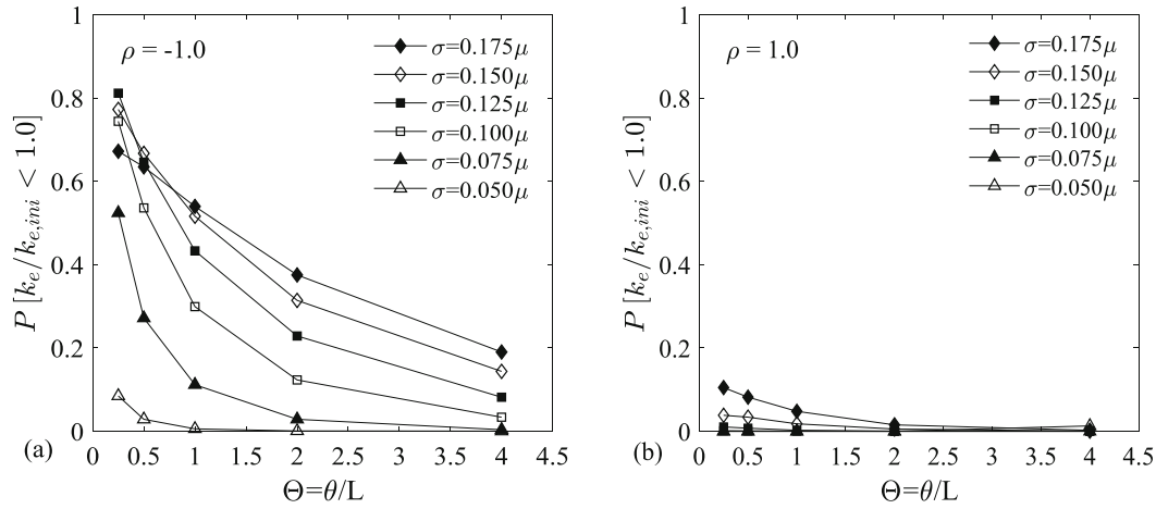
Fig. 1. 1D probabilistic results, comparison of probability of the appearance of blockage during erosion simulations: (a) \rho = -1.0 ; (b) \rho = 1.0
